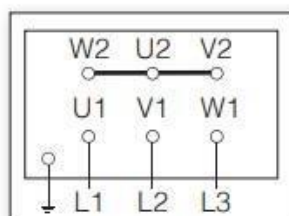
Star Connection
