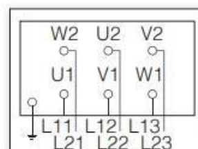
Connection to Star-Delta Starter
