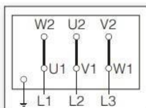
Delta Connection
